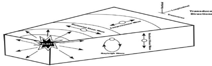
Fig.1. Movement of particles associated with the different wave types
