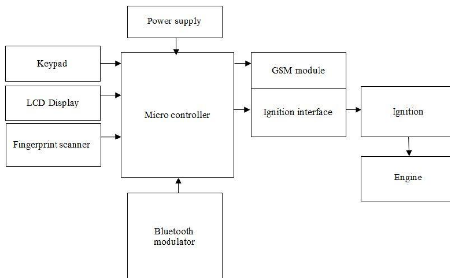
Fig. 2.3 Car Automation
