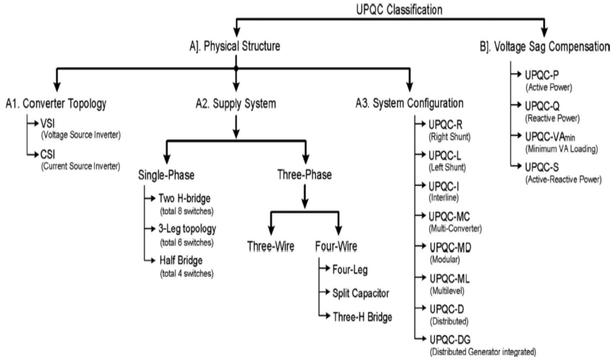
Fig. 5. Classification of UPQC
