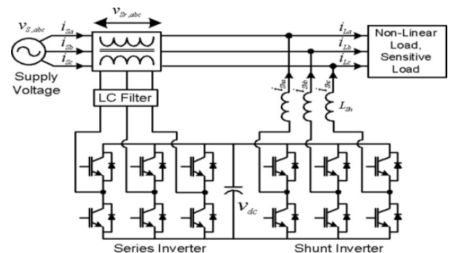
Fig. 8. UPQC of three phases three wires (3P3W)
