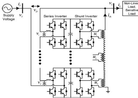
Fig. 12. System configuration of UPQC-Modular
