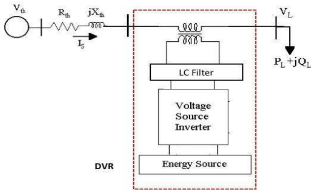
Fig. 2. Dynamic Voltage Restorer (DVR)
