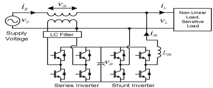
Fig. 7. Configuration of H- Bridge (1P2W)
